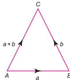
FIGURE 5.11 Case I.
