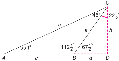
FIGURE 4.15 Example 4.13.
