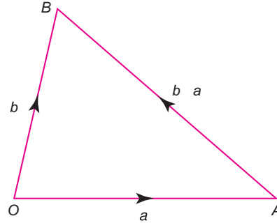
FIGURE 5.10 Theorem 5.6.
