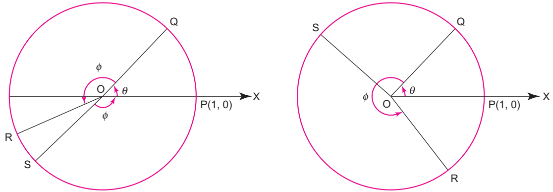
FIGURE 1.34 Case when \theta + \phi > \pi .
