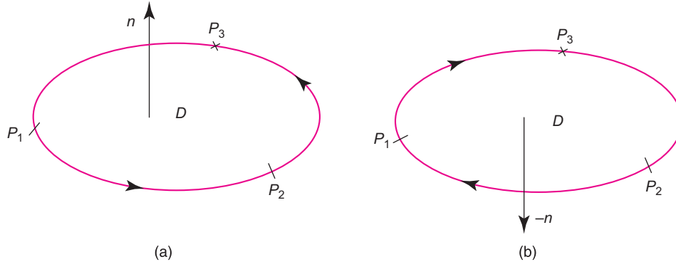
FIGURE 6.19 Orientation of closed curve.
