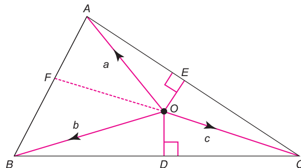
FIGURE 6.8 Theorem 6.10.
