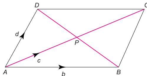
FIGURE 5.24 Theorem 5.16. ■
