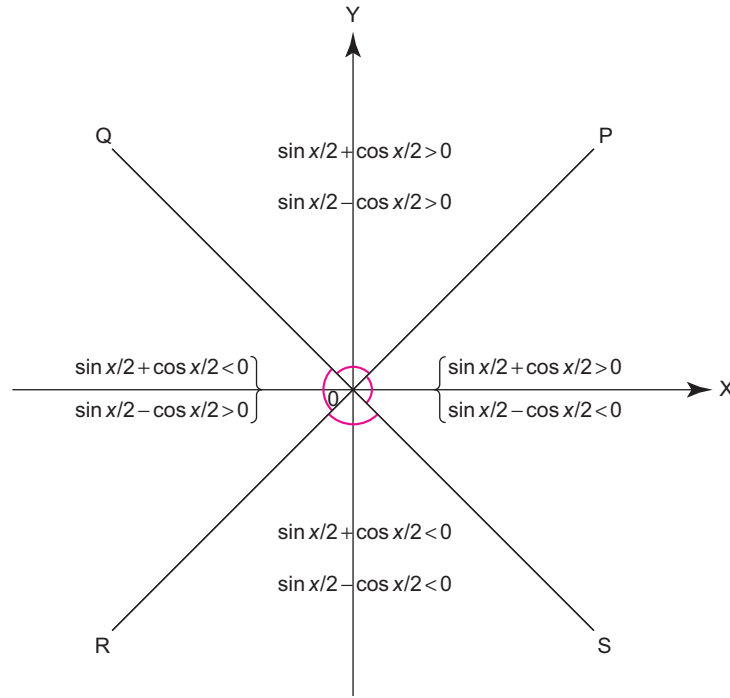
FIGURE 1.35
