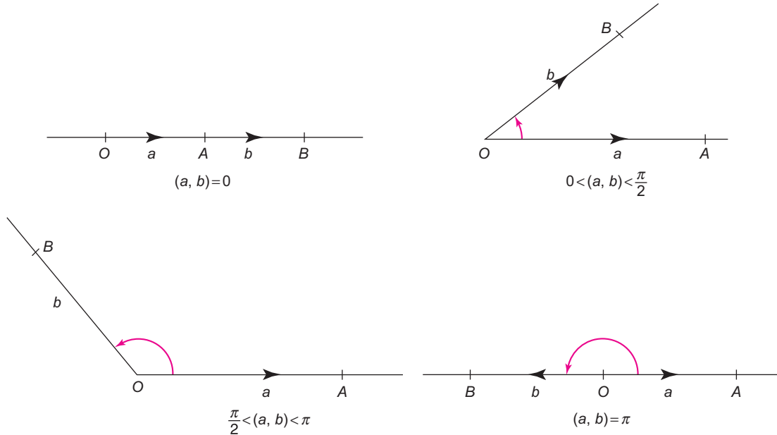
FIGURE 5.28
