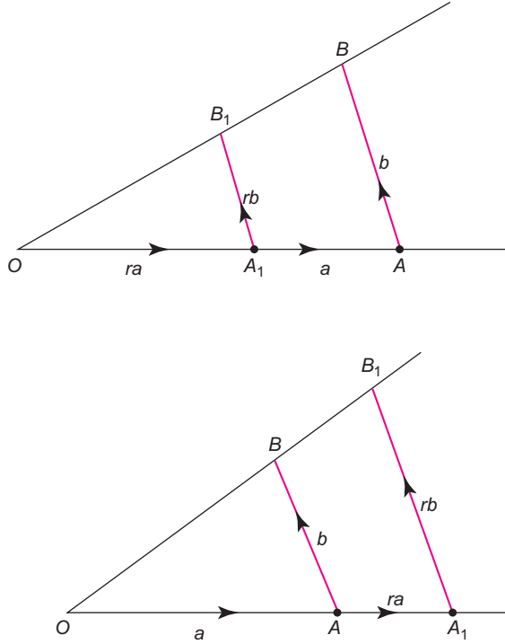
FIGURE 5.17 Theorem 5.11.
